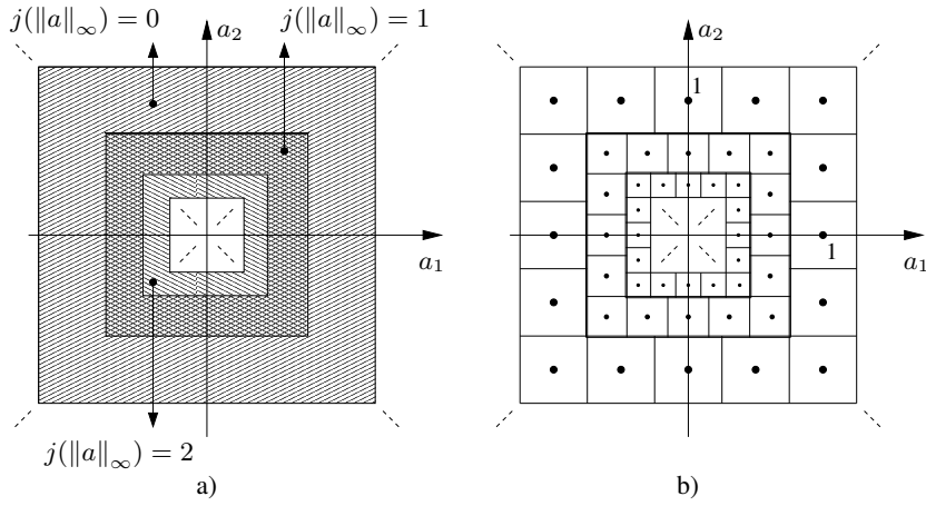
Figure 3.5: The functions a) j(b) and b) \rho^{j(b)} for C = 5 .
