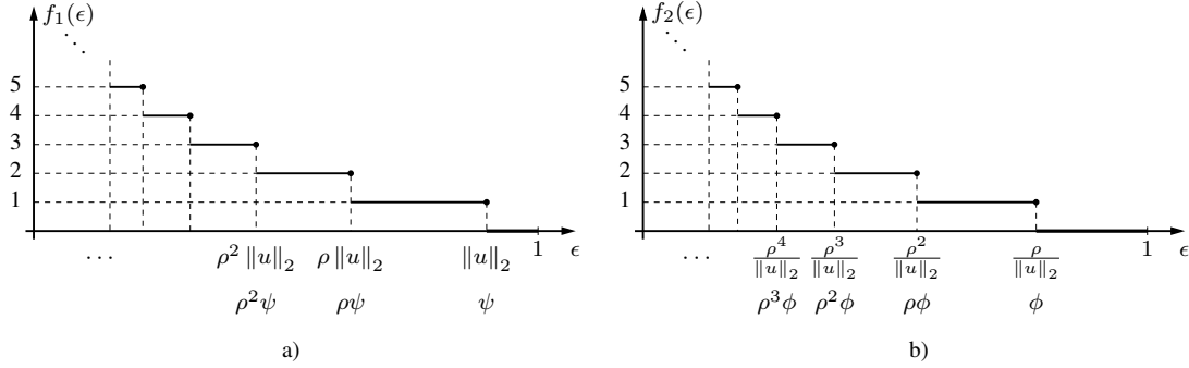
Figure 2.1: The functions f_1 and f_2 defined in (2.39) with u = [0.9 \ 0]^T and \rho = 0.7 . a) f_1 . b) f_2 .
