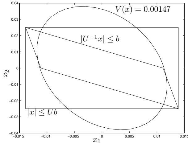
Figure 7.2: Different ultimate bounds in the discretised inverted pendulum
