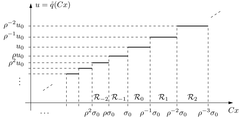
Figure 4.2: Input u = \hat{q}(Cx) as a function of Cx with u_0 = 1 , \sigma_0 = 1.87 and \rho = 0.85 .
