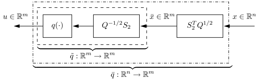
Figure 2.8: Structure of the quantiser \bar{q} in Theorem 2.17.
