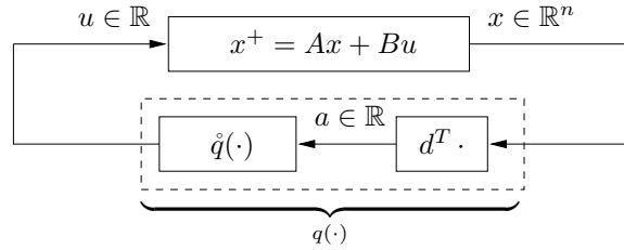
Figure 4.1: The quantised feedback considered: u = q(x) = \dot{q}(d^T x) .
