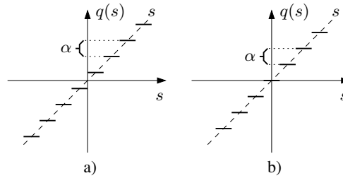
Figure 6.3: Uniform quantisers: a) Midrise. b) Midtread.
