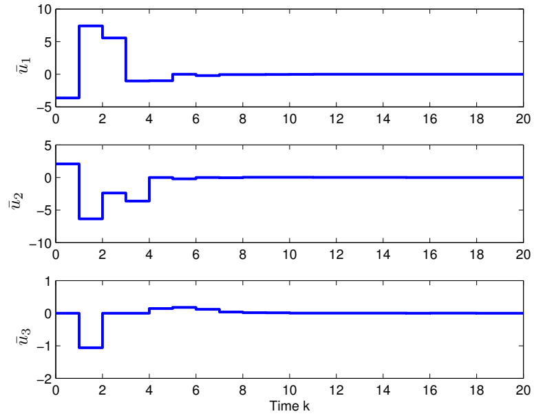
Figure 3.8: Reduced-dimension quantiser output: \bar{u} = \dot{q}(D^T x) .
