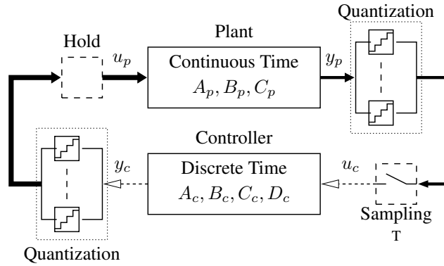
Figure 6.2: Quantised sampled-data control scheme.
