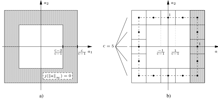
Figure 3.4: a) The set \{a \in \mathbb{R}^2 : j(\|a\|_\infty) = 0\} . b) Values (circles) and regions (solid-line squares) of \hat{q} for a : j(\|a\|_\infty) = 0 , the unit (hyper)cube (dashed line) and the set \{a \in \mathbb{R}^2 : \mathcal{I}(a_1) = 1, j(\|a\|_\infty) = 0\} (shaded).
