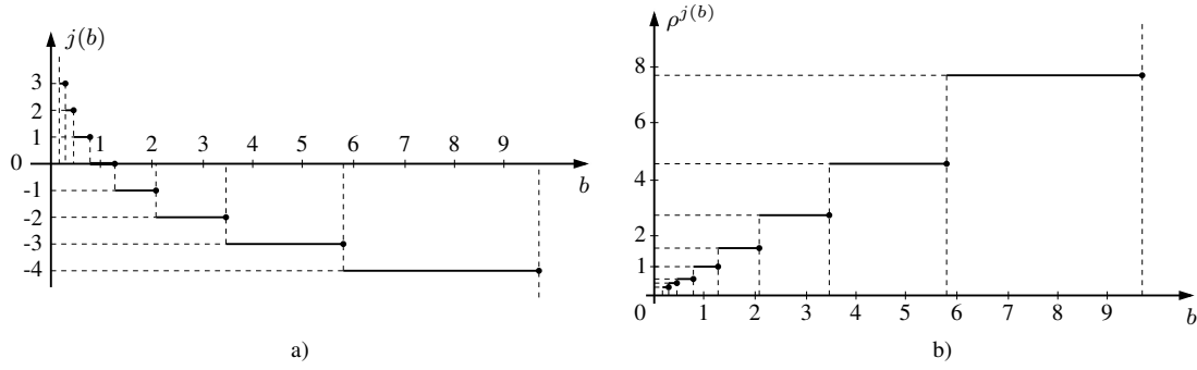
Figure 3.5: The functions a) j(b) and b) \rho^{j(b)} for C = 5 .
