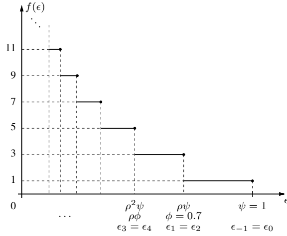
Figure 2.4: f = f_1 + f_2 .
