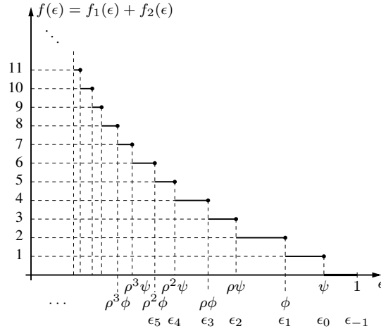
Figure 2.2: The function f defined in (2.33), with u = [0.9 \ 0]^T and \rho = 0.7 .
