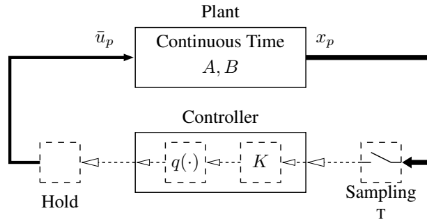
Figure 6.5: Quantised sampled-data system in Ishii et al. (2004).
