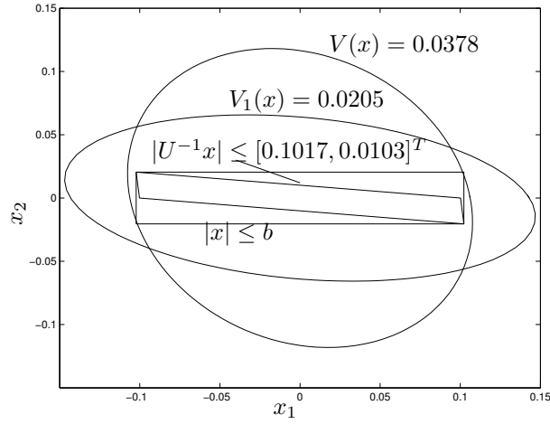
Figure 7.1: Different ultimate bounds in the pendulum system
