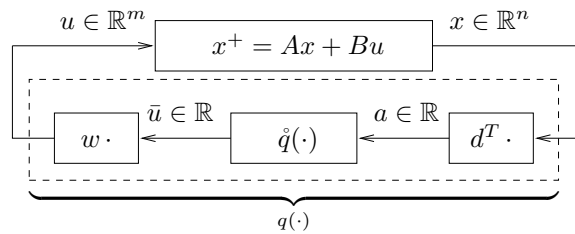
Figure 5.1: The quantised feedback considered: u = q(x) = w\hat{q}(d^T x) .
