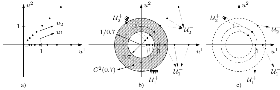
Figure 2.5: a) \mathcal{U}(q) . b) \mathcal{U}_1^+ , \mathcal{U}_2^+ , \mathcal{U}_1^- , \mathcal{U}_2^- and C^2(0.7) . c) \mathcal{U}(q) \cap C^2(0.7) .
