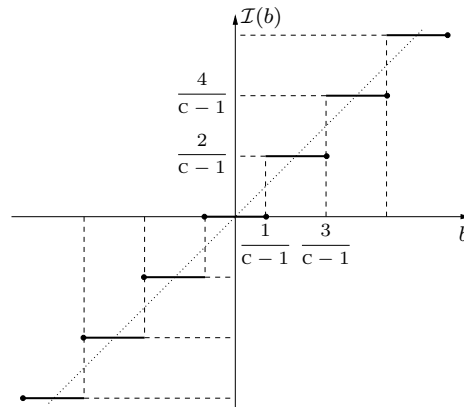
Figure 3.3: The function \mathcal{I} : \mathbb{R} \rightarrow \frac{2}{C-1}\mathbb{Z} .
