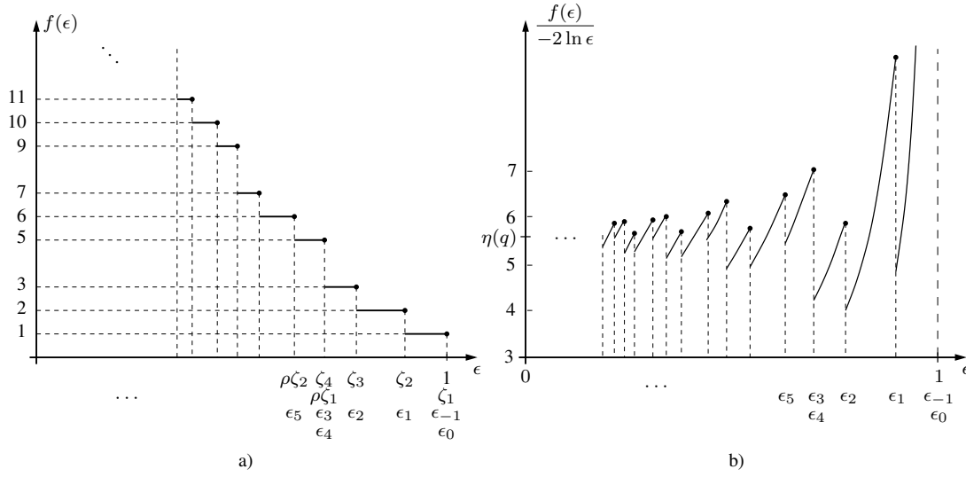
Figure 2.6: a) The function f(\epsilon) . b) f(\epsilon) / -2 \ln \epsilon .
