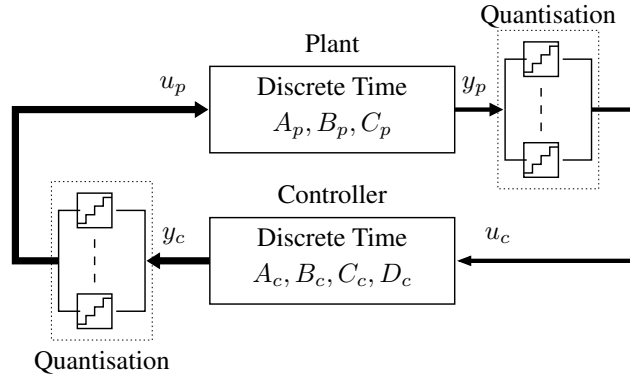
Figure 6.1: Quantised discrete-time control scheme.
