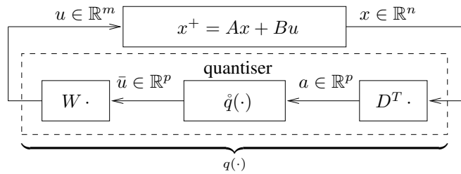
Figure 3.1: The quantised feedback considered: u = q(x) = W \mathring{q}(D^T x) .
