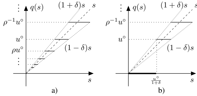
Figure 6.4: a) Logarithmic quantiser. b) Semitruncated logarithmic quantiser.
