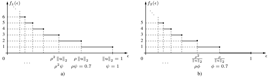
Figure 2.3: The functions f_1 and f_2 defined in (2.39) with u = [\sqrt{2}/2 \ \sqrt{2}/2]^T and \rho = 0.7 . a) f_1 . b) f_2 .
