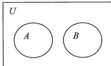
A \cap B = \emptyset
